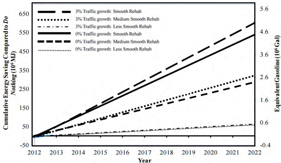
Figure 7. Payback time in MJ and equivalent gallons of gasoline for a high volume interstate route over 10-year analysis period for three percent slab replacement and diamond grinding of all lanes versus leaving the pavement rough, considering three levels of constructed smoothness (Wang et al. 2012).
