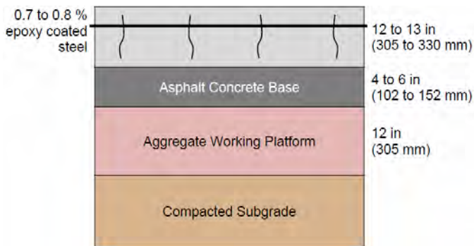
Figure 3. Example of longer life CRCP design.
