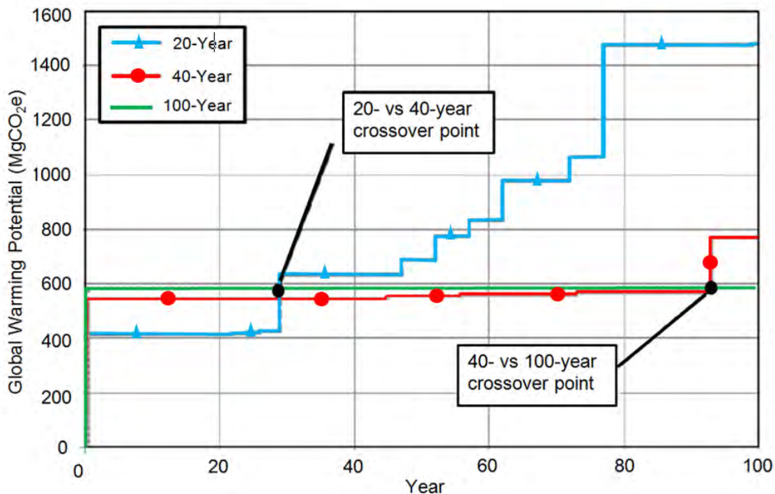
Figure 6. Example of payback time analysis considering only the material production and construction phases of three different pavement design lives (modified from Santero 2009).
