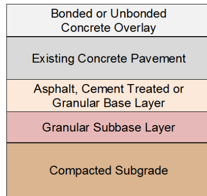
Figure 4. Cross section of concrete pavement structures rehabilitated with overlays (not to scale).
