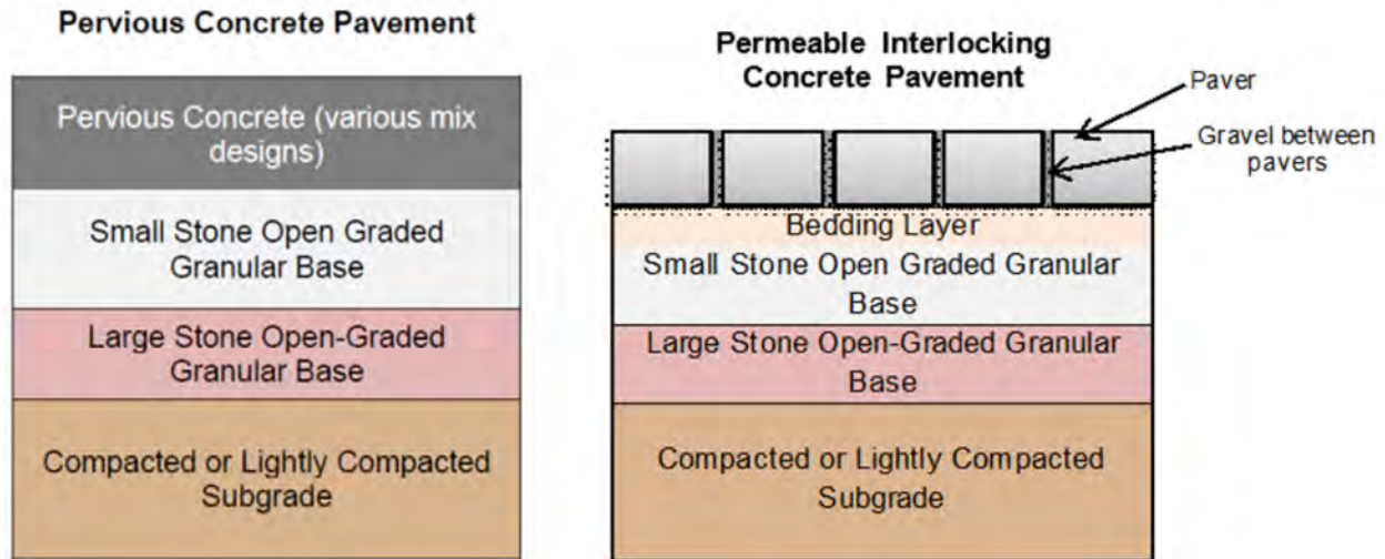
Figure 5. Examples of fully permeable concrete pavement systems.
