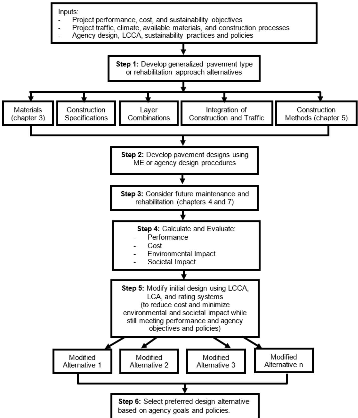
Figure 2. Overall process for considering sustainability in pavement design. (Note: Chapter numbers refer to the chapter in FHWA-HIF-15-002 [FHWA 2015]).
