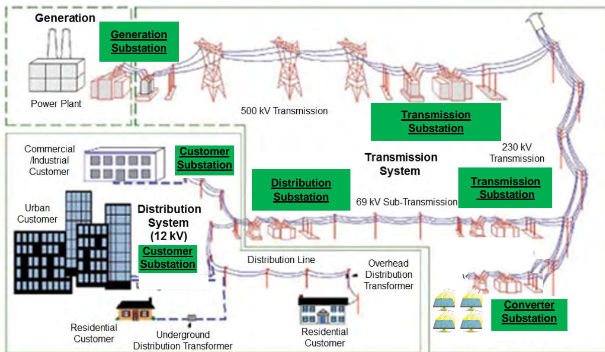
Figure 1: Electric Power System with Substation Categories
