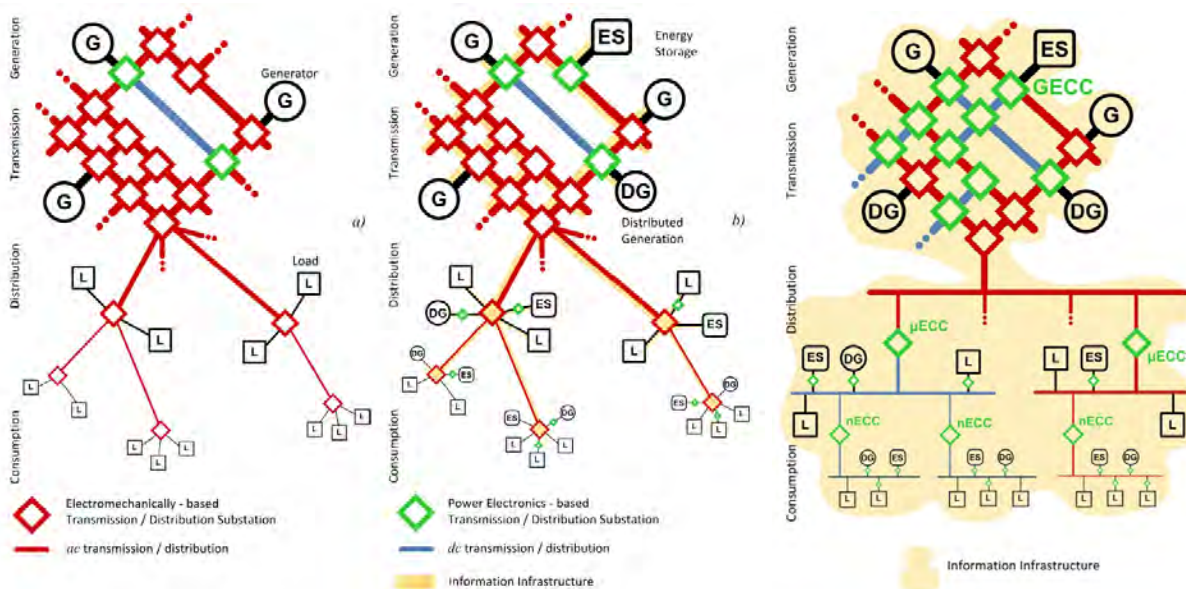
Figure 12: Potential Evolution of Grid Topologies and Architectures 63
