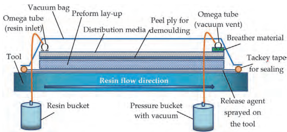
Figure 5. The schematic of the VARTM process.
