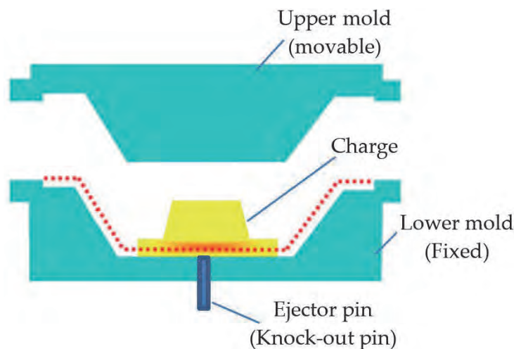
Figure 7. The schematic of compression moulding process.
