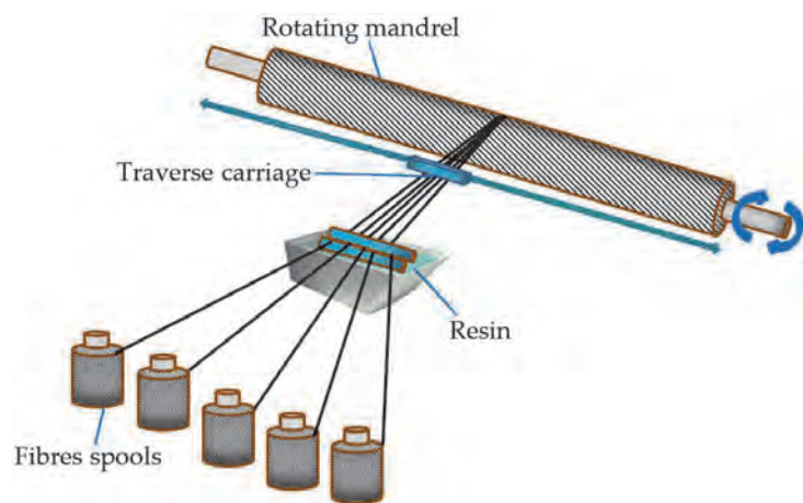
Figure 9. The schematic of the filament winding process.
