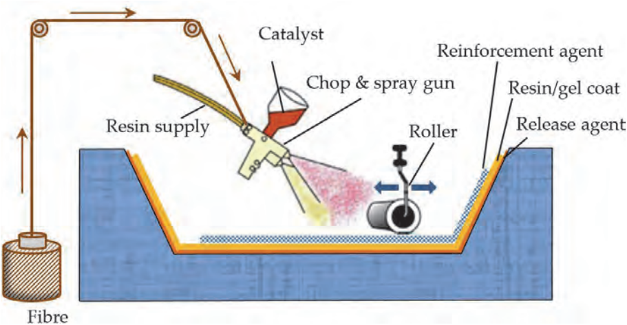
Figure 3. The schematic of the spray lay-up process.
