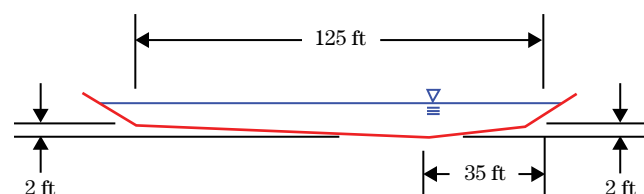
Figure 8 Sand channel cross section
