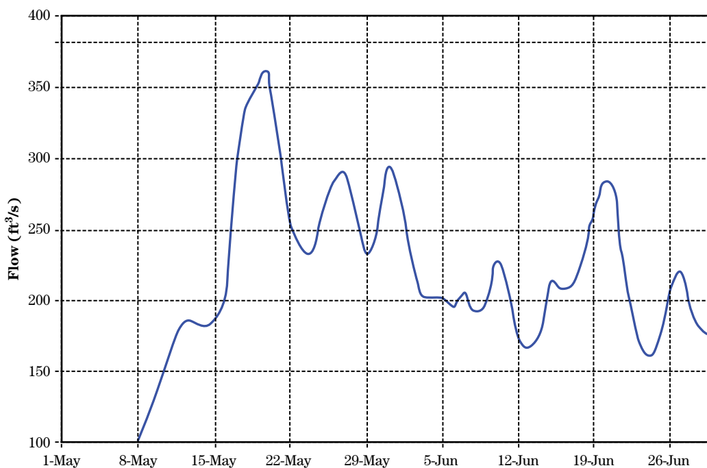
Figure 16 Seasonal hydrograph
