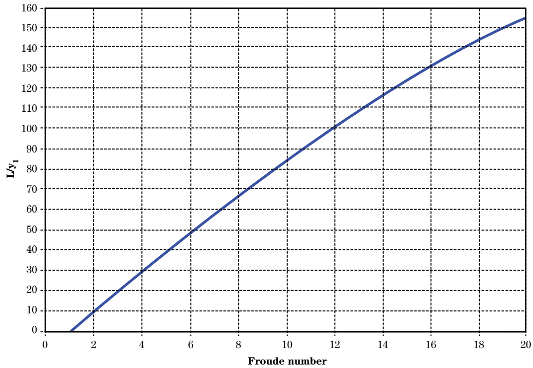
Figure 20 Determination of jump length based on upstream Froude number
