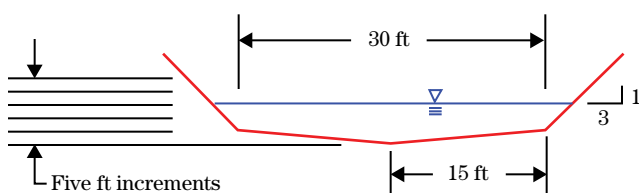
Figure 3 Problem cross section
