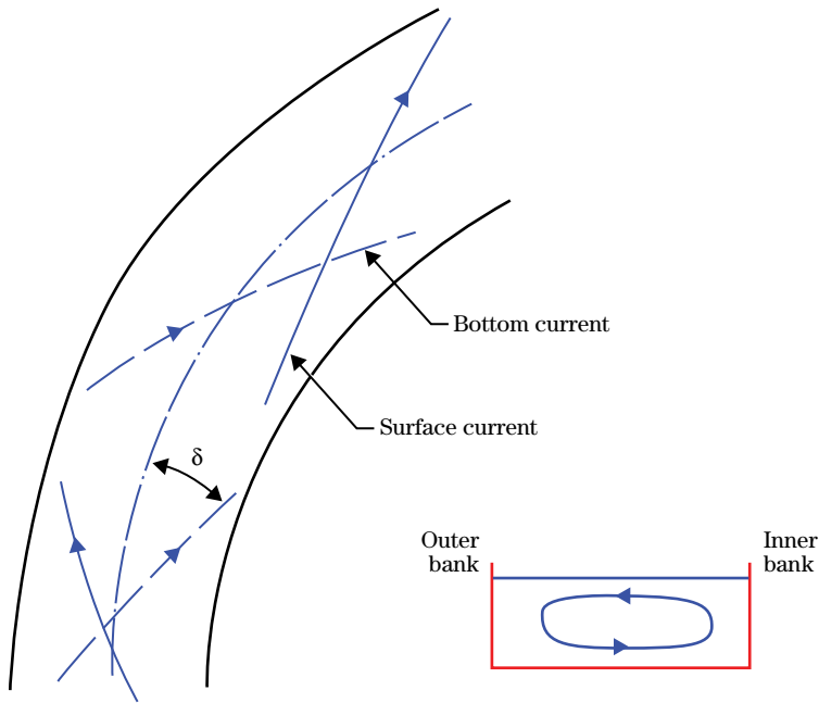
Figure 12 Spiral flow characteristics for a typical reach
