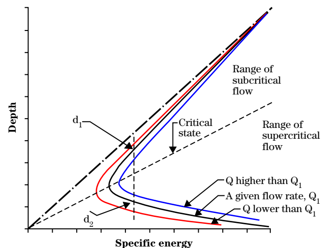
Figure 2 Specific energy vs. depth of flow
