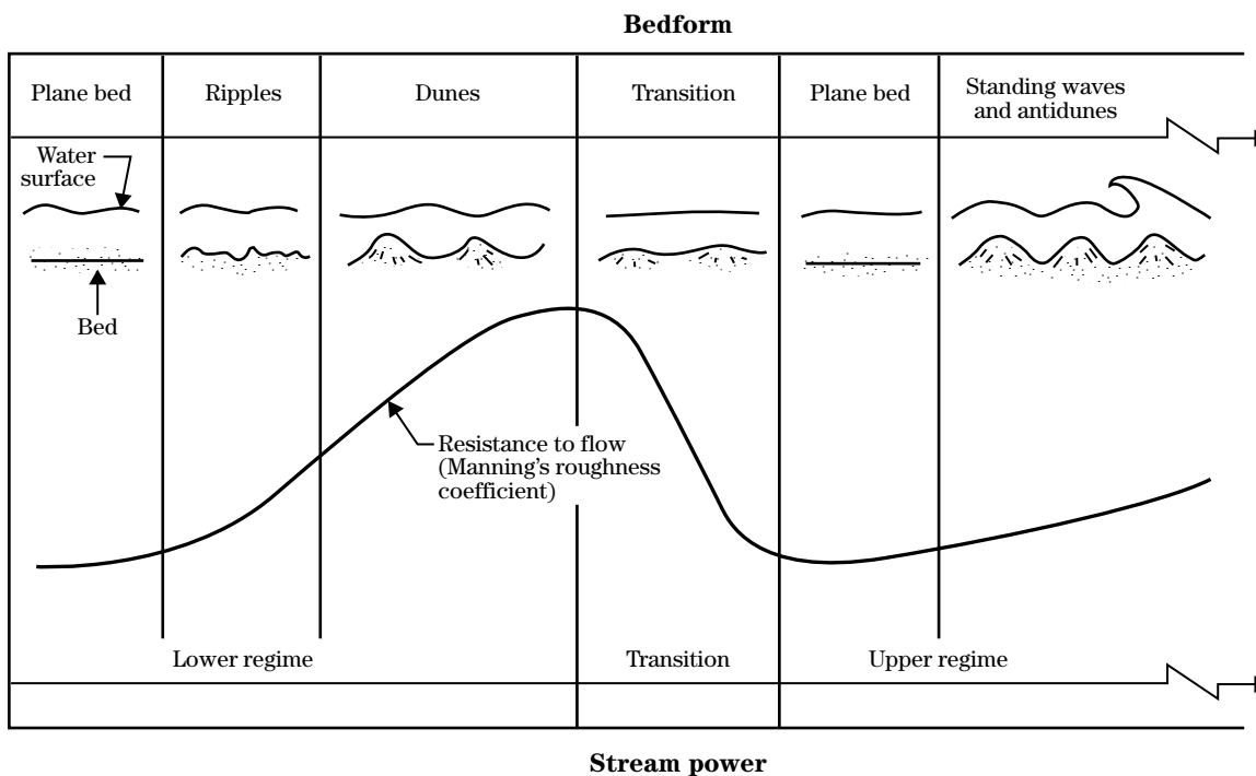
Figure 10 General bedforms for increasing stream power
