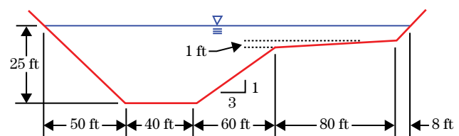
Figure 5 Cross-sectional dimensions
