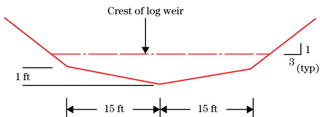
Figure 18 Problem determinations for determination of log weir
