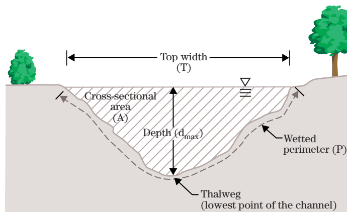
Figure 1 Channel cross-sectional parameters (per ft of channel length)
