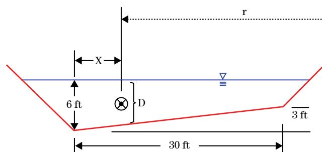
Figure 14 Channel centerline at centroid of flow \otimes
