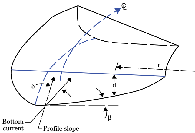
Figure 13 Flow characteristics for a typical reach
