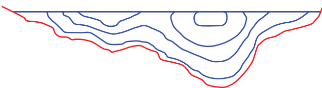
Figure 11 Flow velocities for a typical cross section
