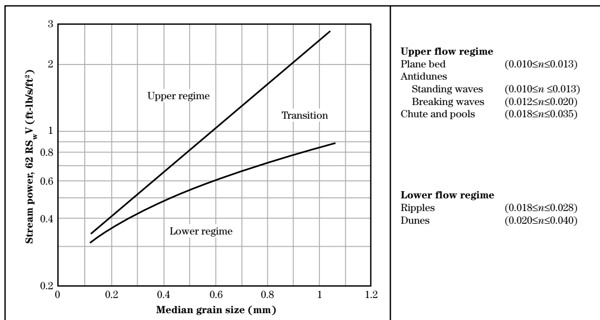
Figure 9 Plot of flow regimes resulting from stream power vs. median fall diameter of sediment
