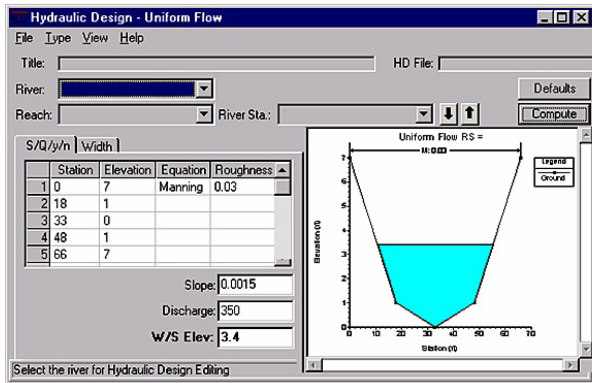
Figure 4 HEC-RAS screen shot for uniform flow computation
