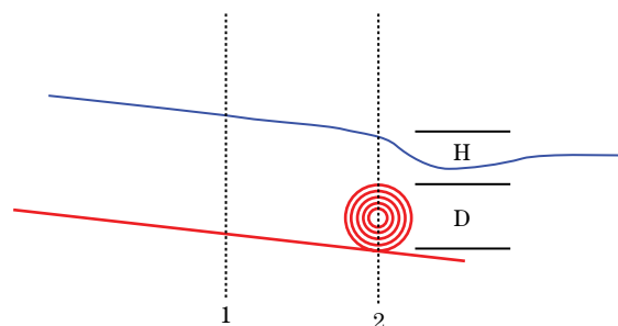
Figure 19 Profile for crest of log weir problem
