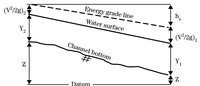
Figure 17 Standard step method
