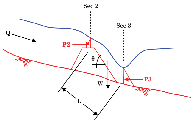
Figure 21 Parameters involved with modeling a hydraulic jump
