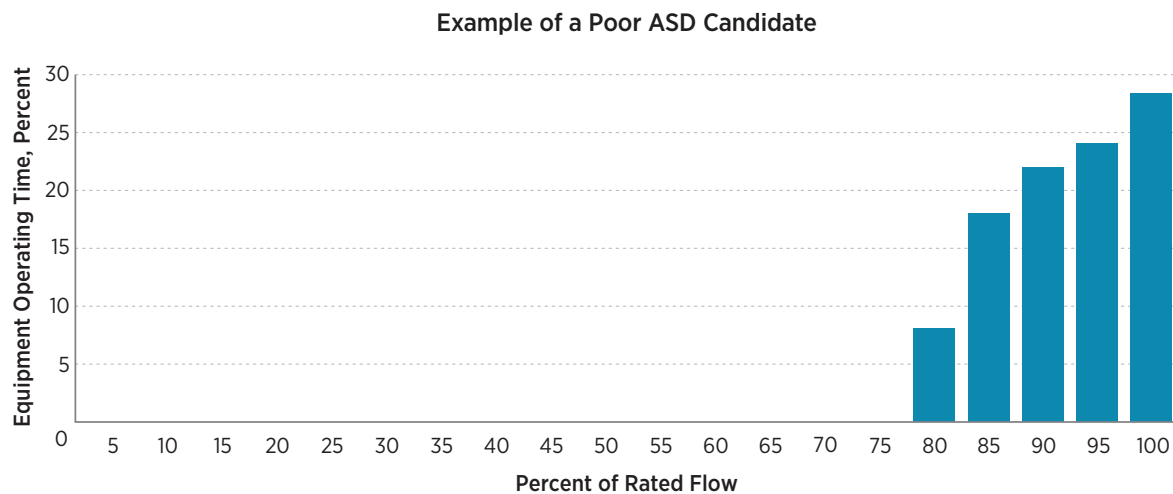
Figure 8-14. A Load Profile that Indicates a Poor ASD Retrofit Opportunity
