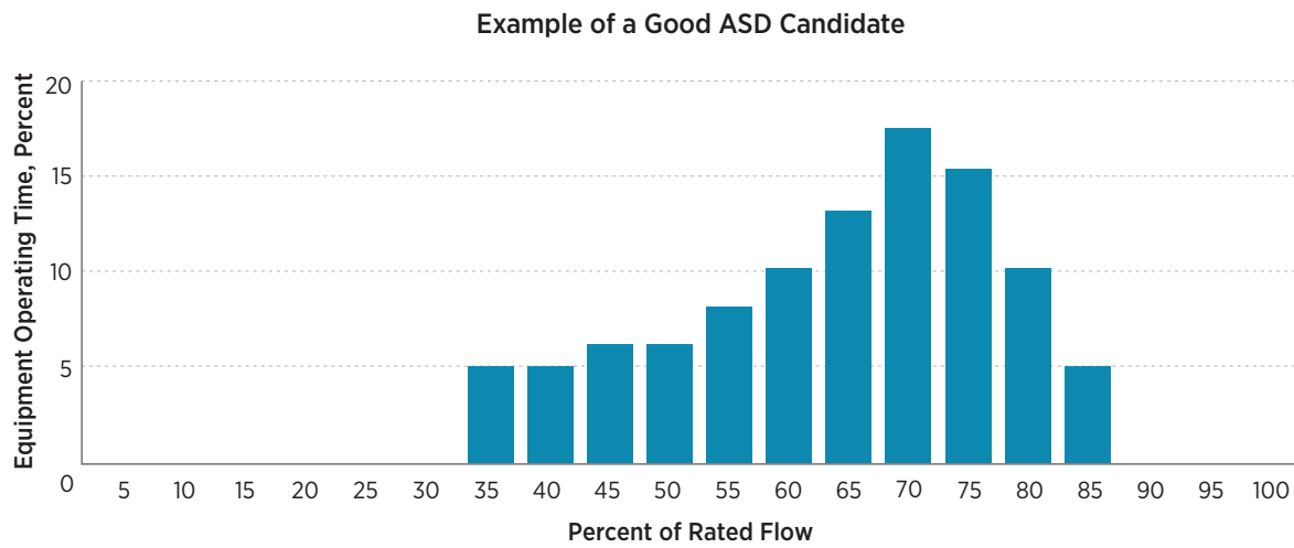
Figure 8-13. A Load Profile that Indicates a Good ASD Retrofit Opportunity
