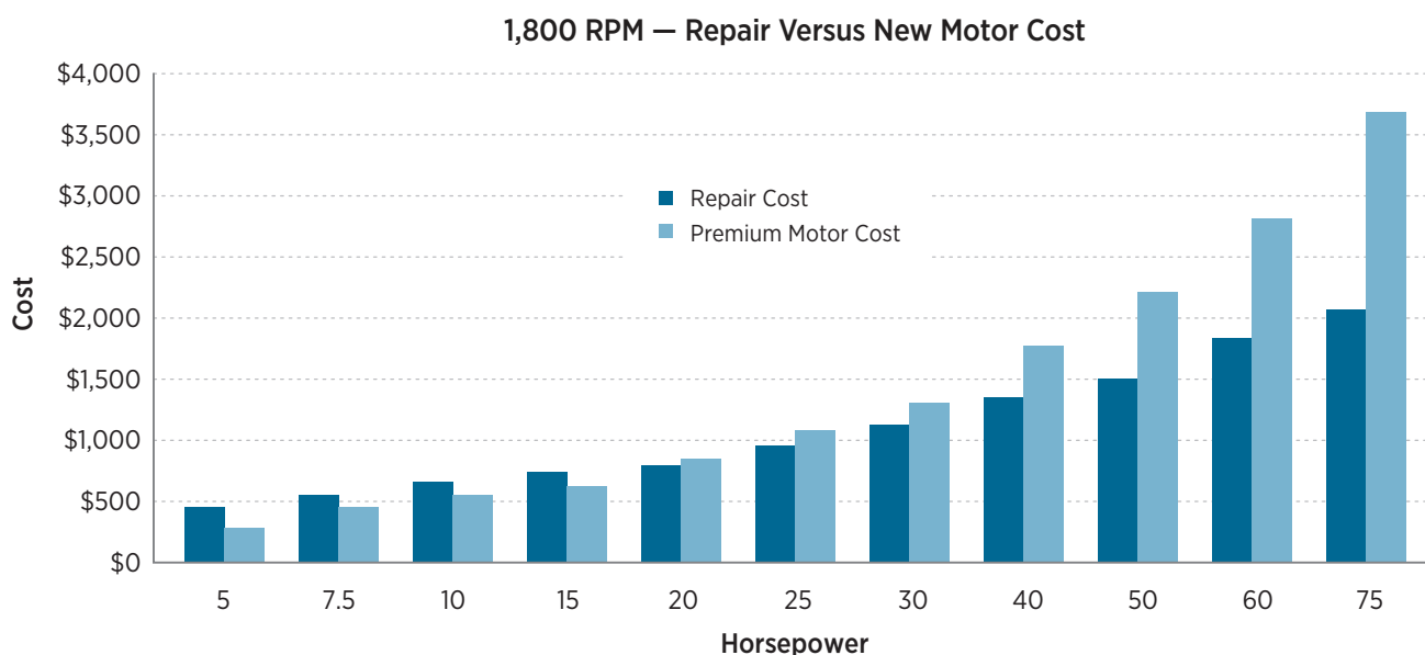
Figure 7-1. Repair and New Premium Efficiency Motor Costs (for 1,800 RPM TEFC Motors, 2011
