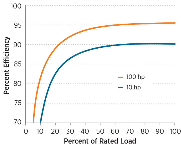
Figure 8-16. Motor Efficiency Versus Load Curves
