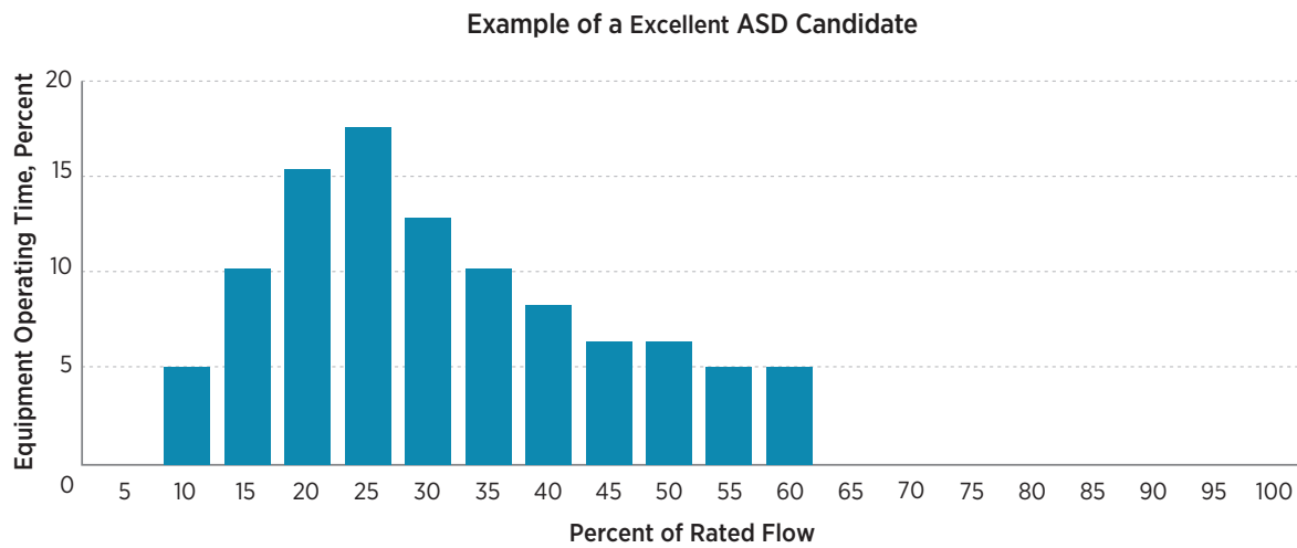
Figure 8-12. A Load Profile that Indicates an Excellent ASD Retrofit Opportunity
