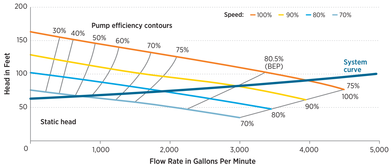
Figure 8-11. System Curve with a Static Head Requirement
