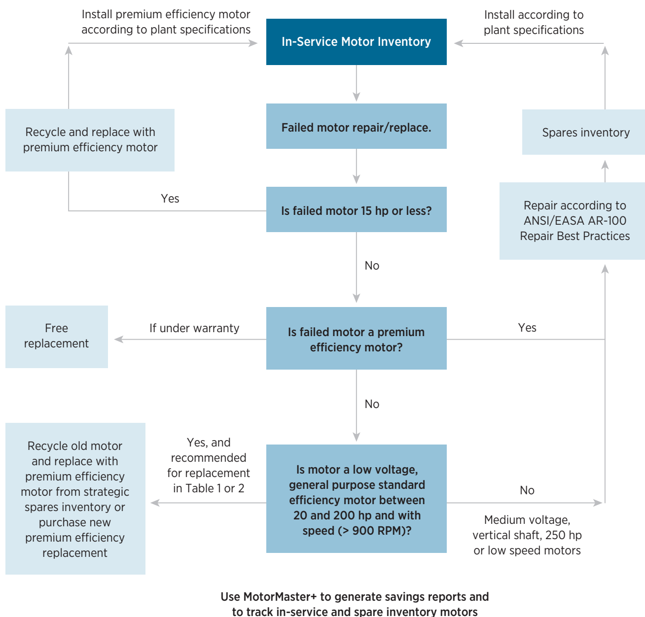
Figure 7-7. Sample Repair Versus Replace Decision Path for General Purpose Motors
