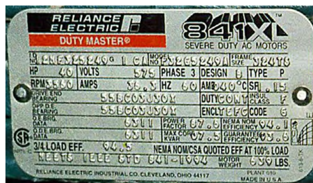
Figure 3-1. Motor Nameplate. Photo from Baldor Electric
