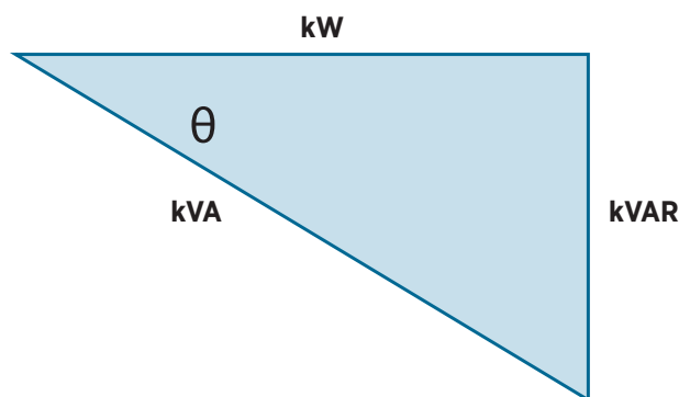
Figure 9-1. The Power Triangle
