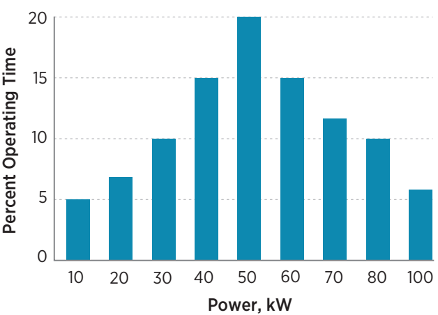
Figure 5-2. Power Logging Data Displayed in Histogram Format
