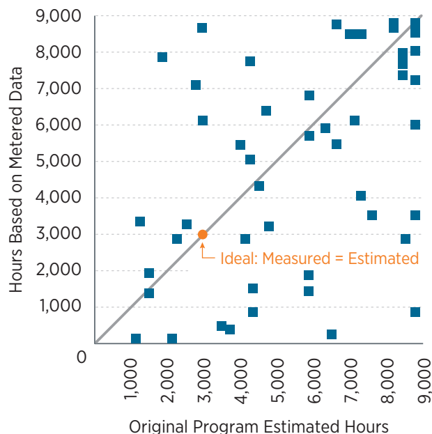
Figure 3-3. Operating Hour Assumptions Versus Measured Values
