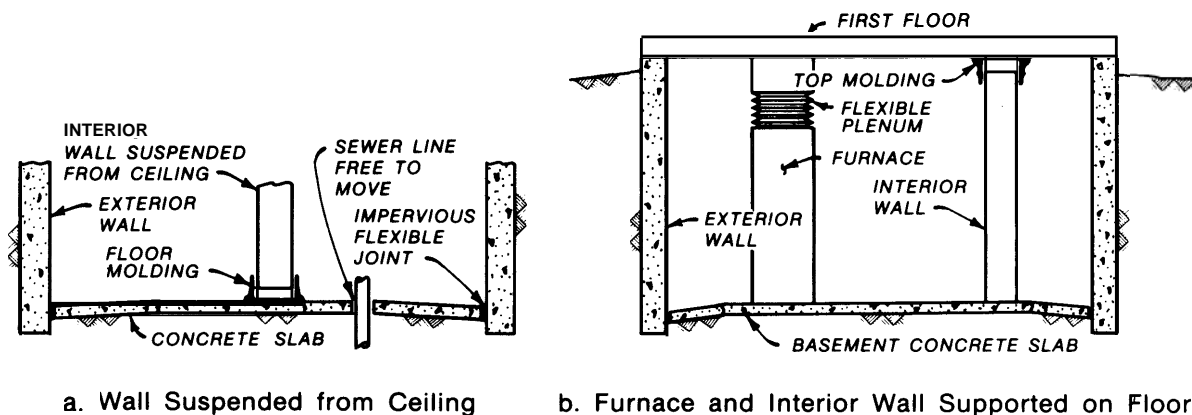
Figure 6-3. Interior joint details for slab-on-grade.
