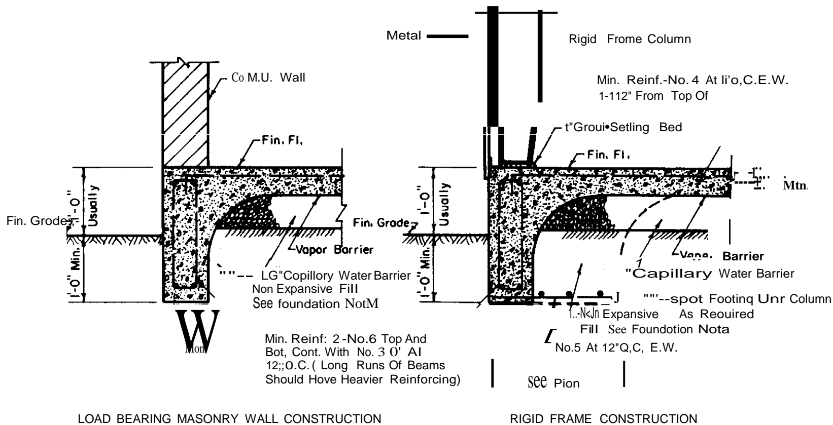
Figure C-9. Typical ribbed mat foundations.
