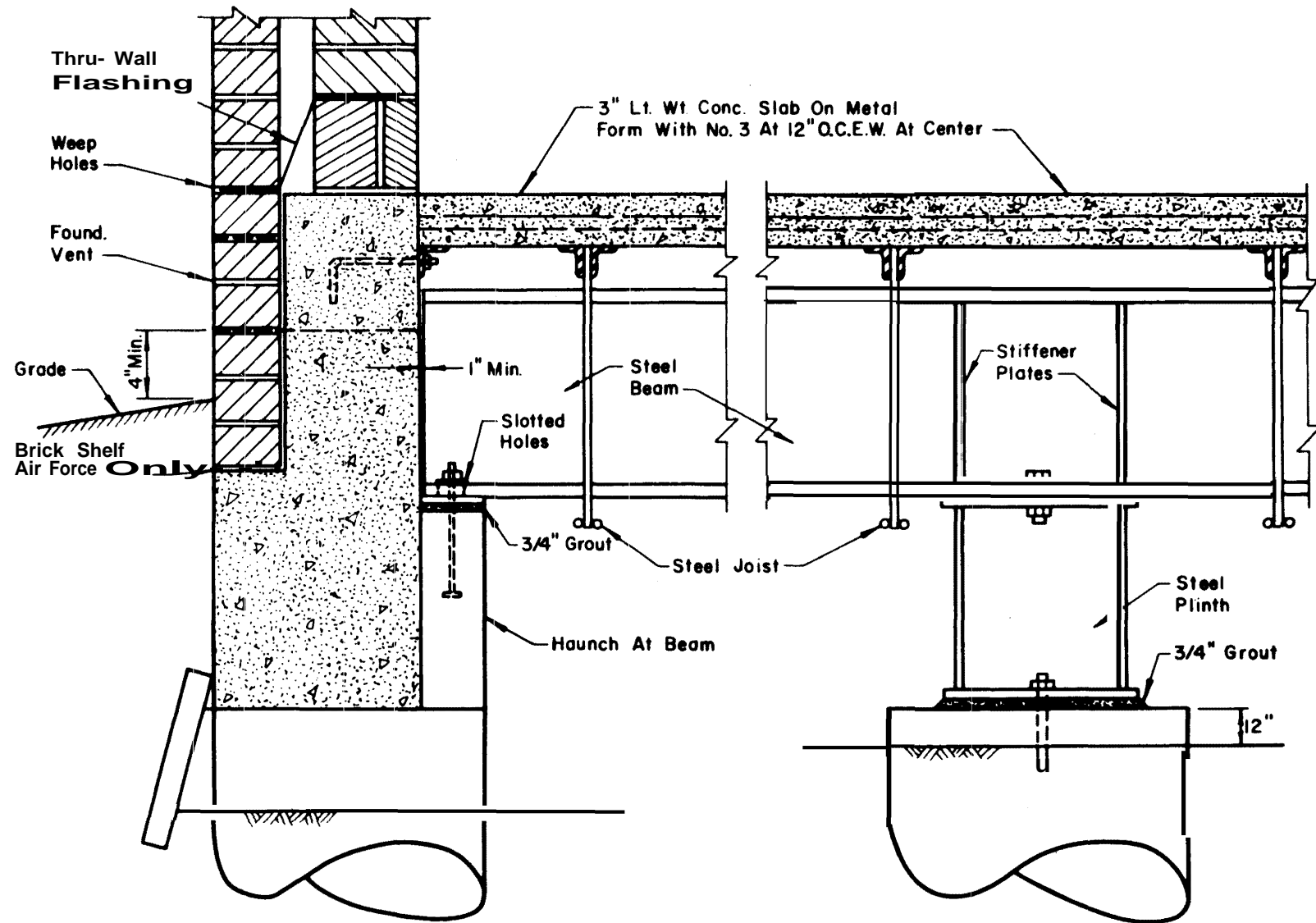
Figure C- 7. Typical bar joist first floor framing.
