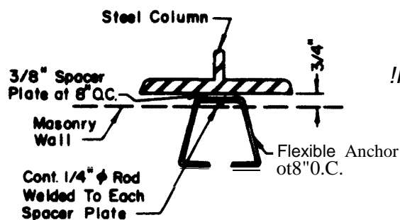
FLEXIBLE ANCHOR
