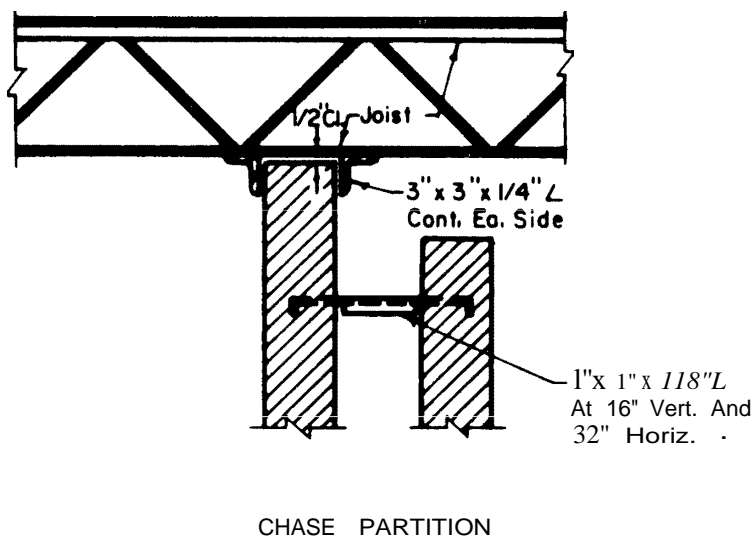
Figure C-6. Typical details of interior partitions.
