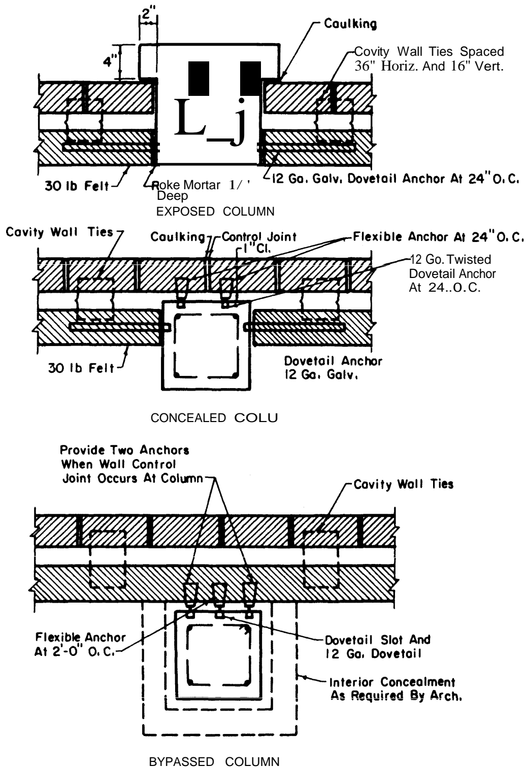
Figure C-2. Wall ties to concrete column.
