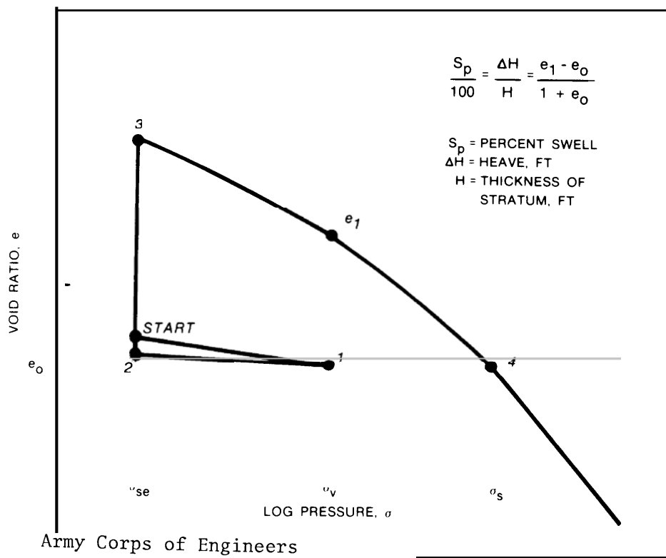
Figure 4-2. Simple swell test.
