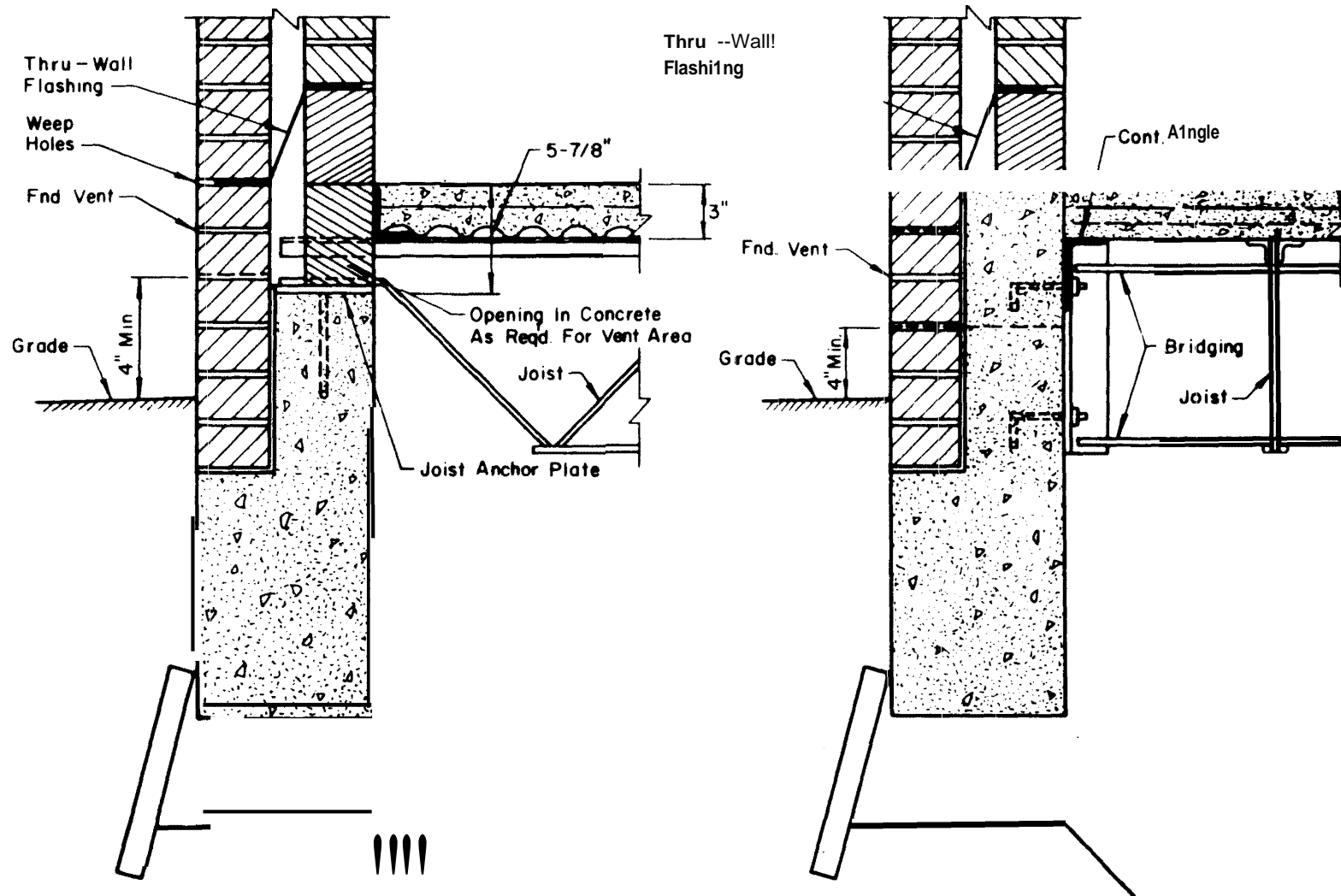
Fig C-8. Typical cast-in-place or precast concrete grade beam with steel bar joist floor framing.
