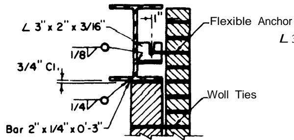
WALL ANCHORAGE TO STEEL BEAM IE
