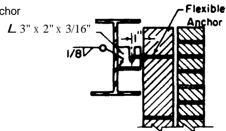
WALL ANCHORAGE TO STEEL BEAM IE
