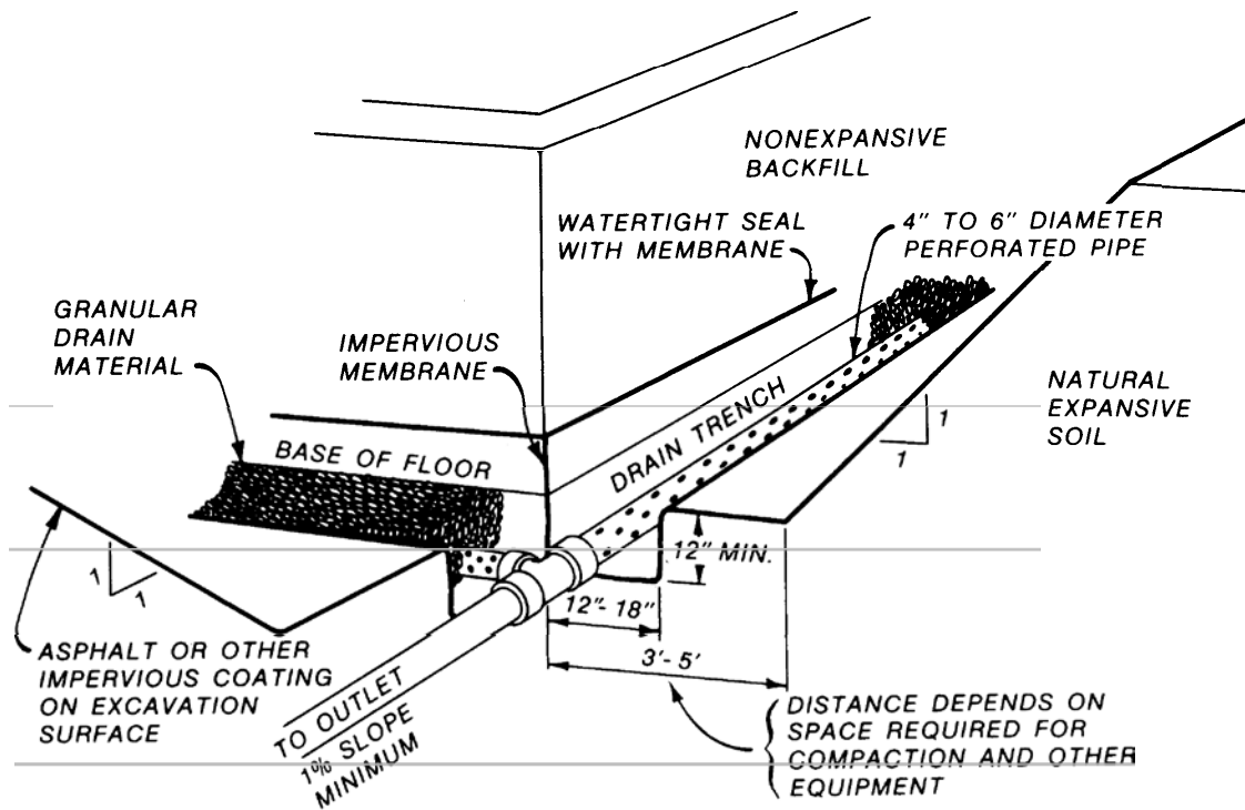
Figure 7-1. Drainage trench around outside of structure.
