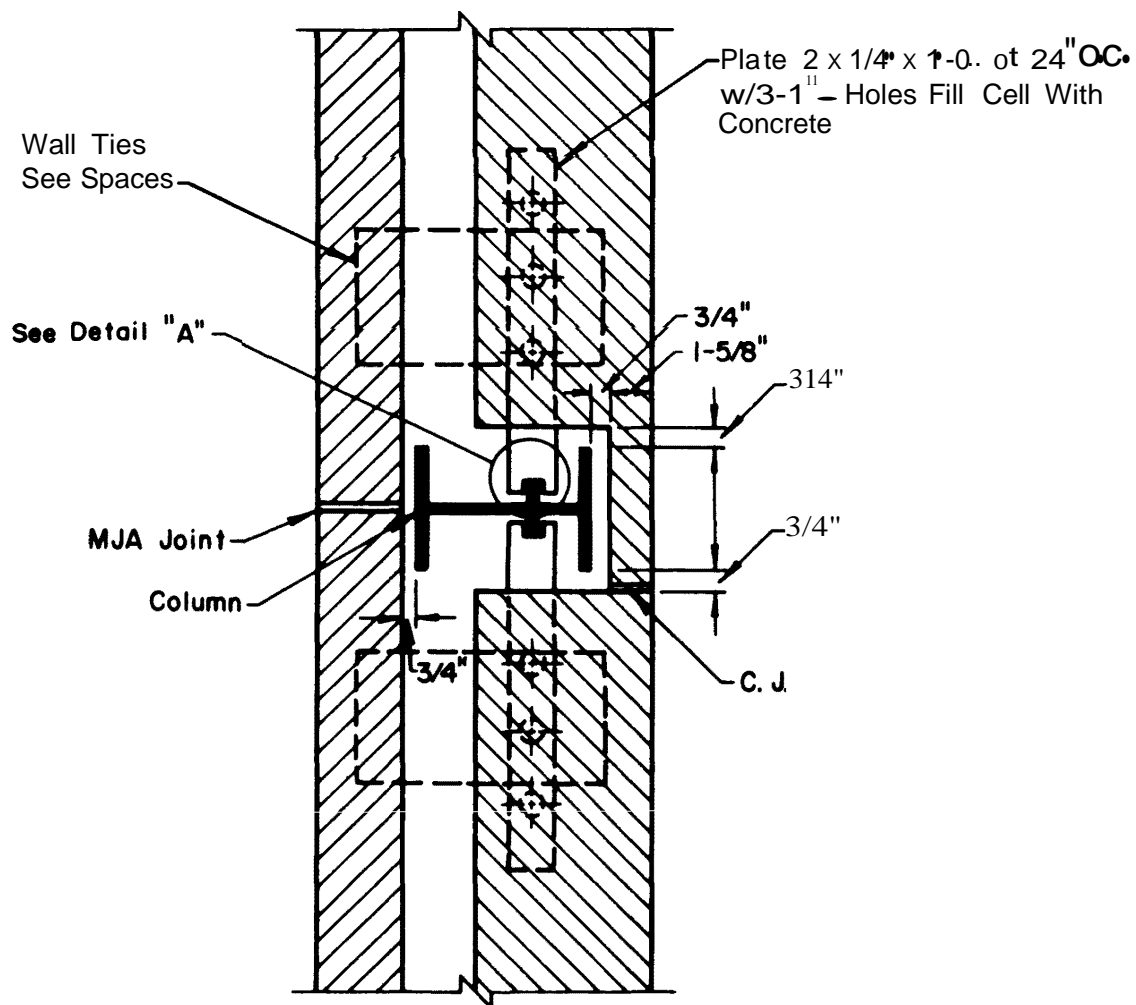
Figure C-3. (Sheet 2 of 2).
