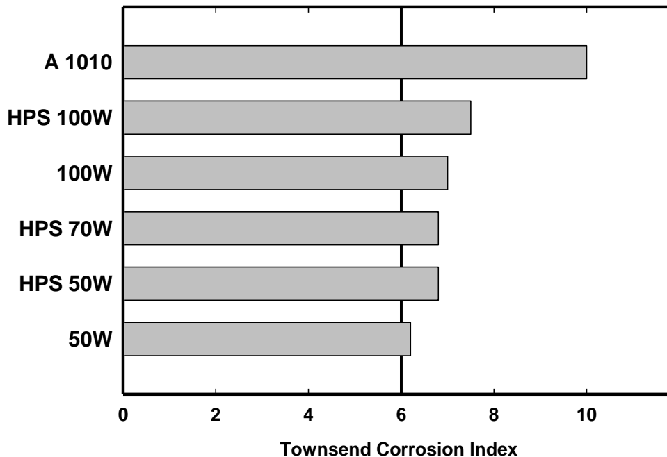
Figure 14 Comparison of the typical corrosion index between different grades of weathering steels based on the Townsend corrosion index.
