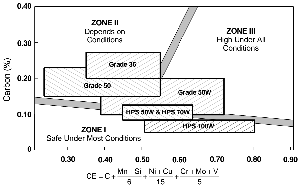
Figure 12 Graville weldability diagram to indicate the relative susceptibility to HAZ cracking of bridge steels.
