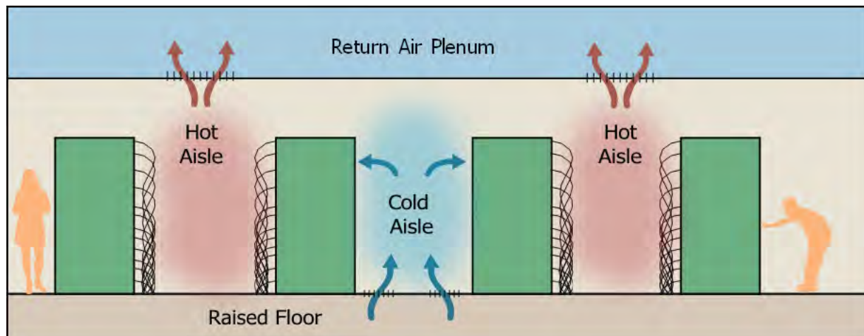
Figure 4-1. Example of a hot aisle/cold aisle configuration
